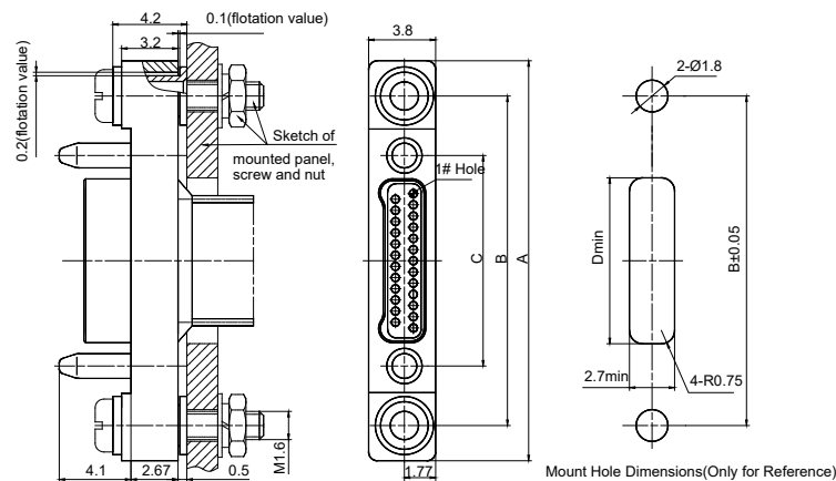
Plug
