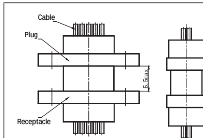
mating drawing
